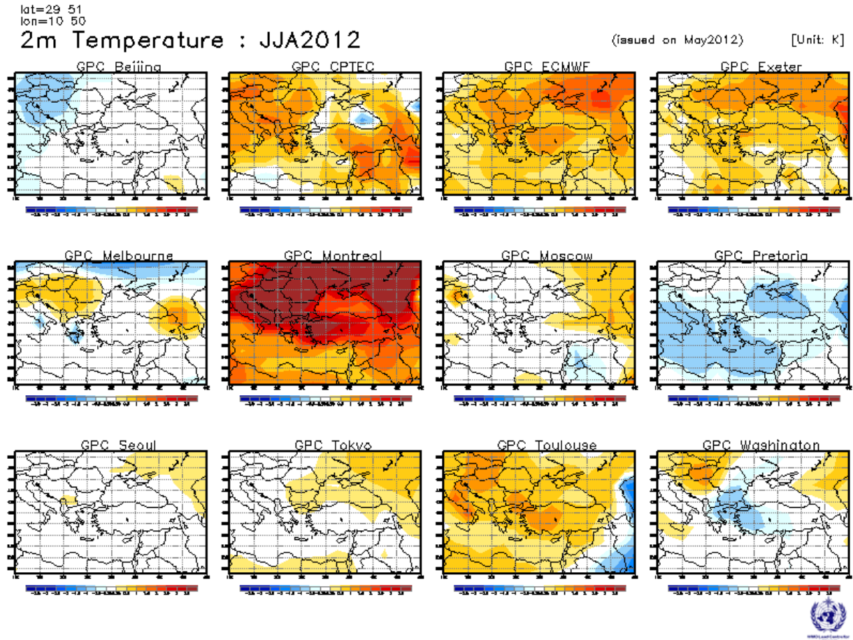
FIG. 1: GPC's forecasts for JJA 2012 temperature anomaly.
