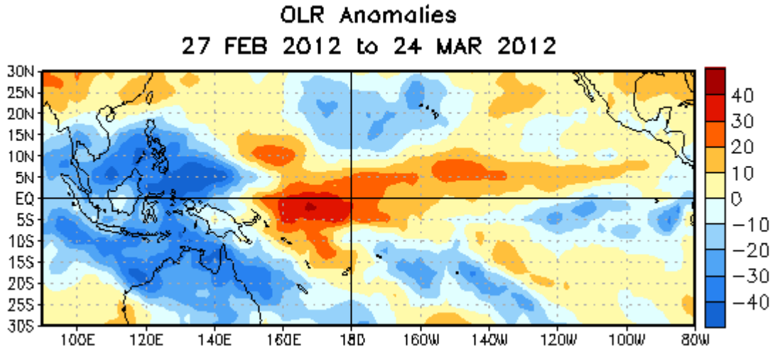
Figure 6. Average outgoing longwave radiation (OLR) anomalies ( \text{W/m}^2 ) for the four-week period 27 February – 24 March 2012. OLR anomalies are computed as departures from the 1979-1995 base period pentad means.
