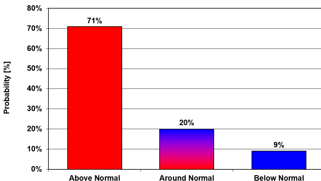
Fig 1: The temperature (at 2m above ground) probability for JJA 2023 terciles over Israel.
