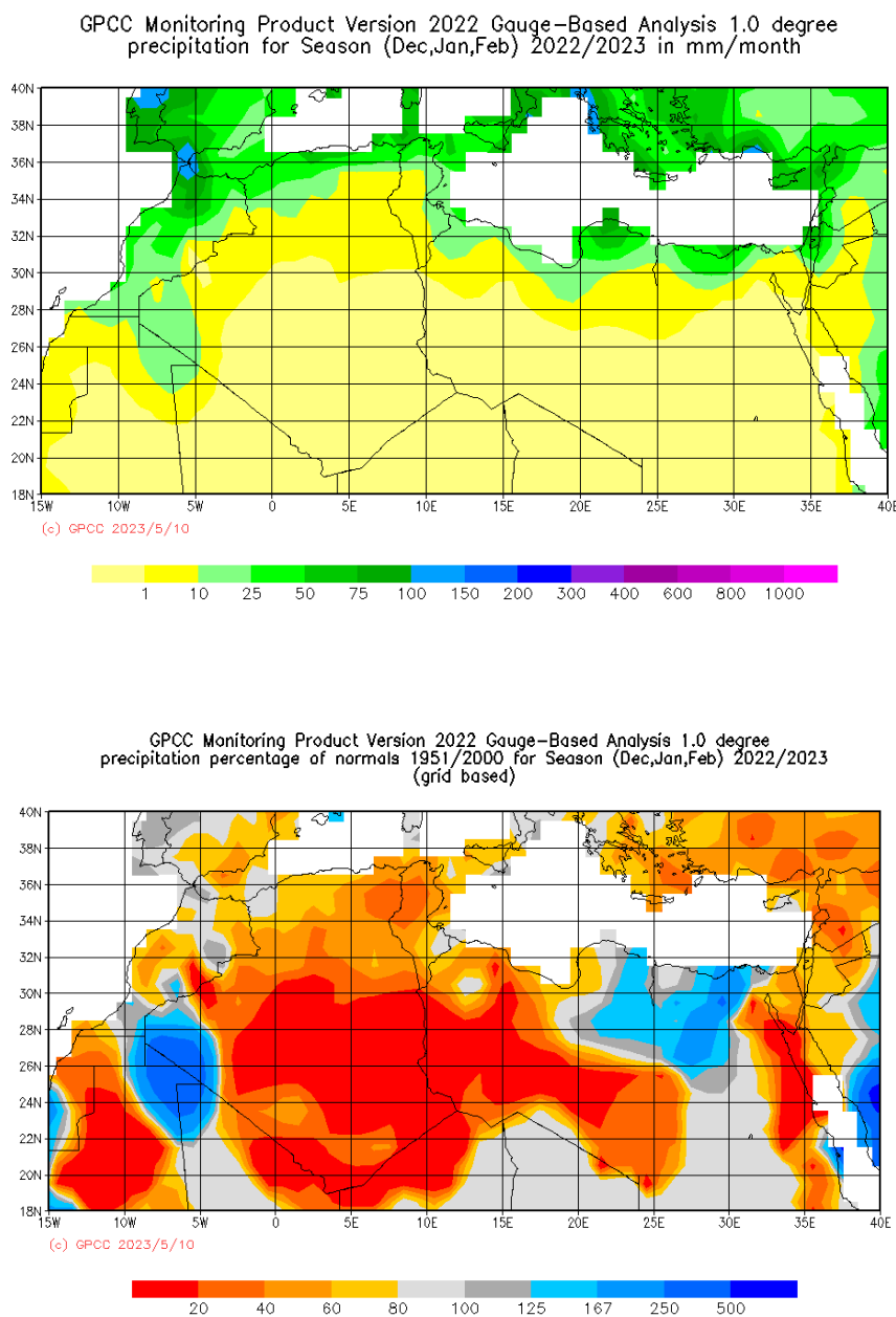
Figure 18: Winter (DJF 2022/23) precipitation totals and anomalies. Source: Global Precipitation Climatology Centre (GPCC), http://gpcc.dwd.de/
