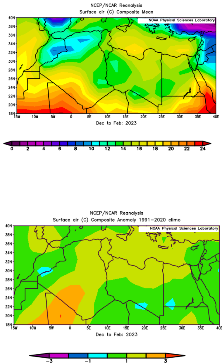
Figure 14: Winter (DJF 2022/23) mean temperatures and anomalies. Source: NOAA Physical Science Laboratory, https://psl.noaa.gov/cgi-bin/data/composites/printpage.pl
