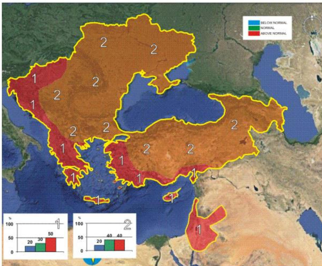
Fig 1. SEECOF-26 temperature outlook for 2021-2022.
