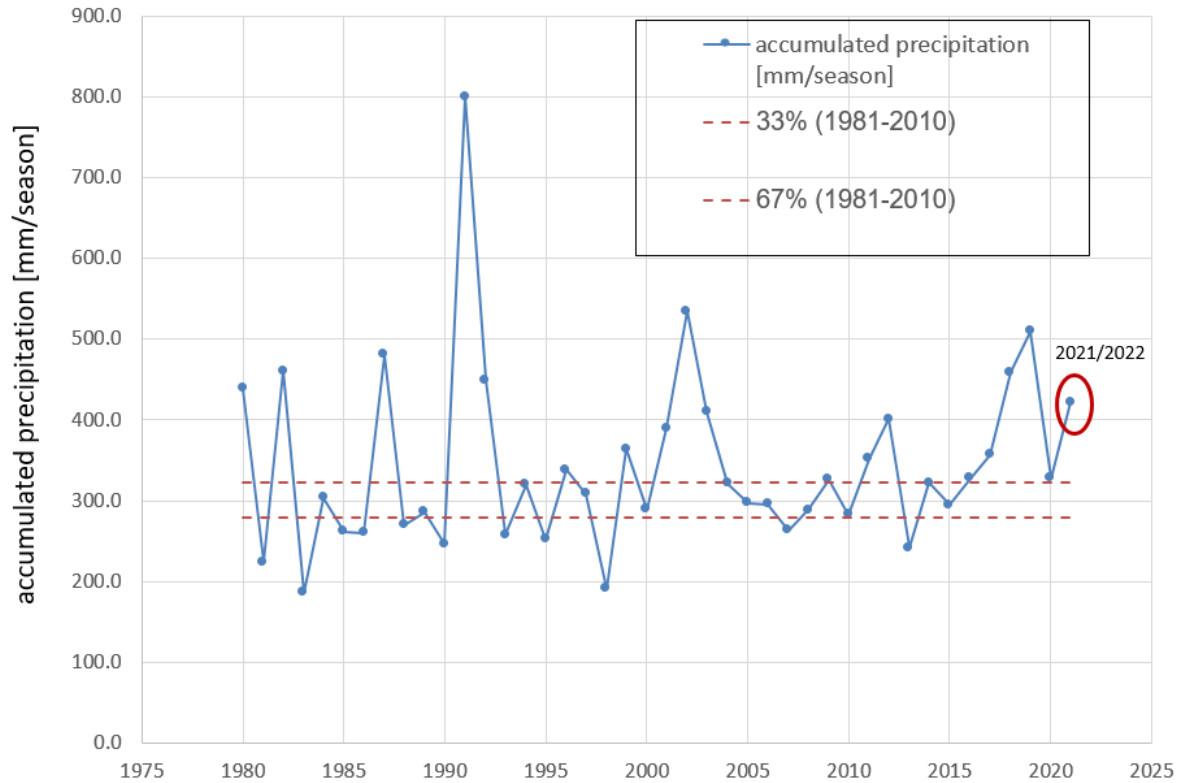
Fig 4. DJF accumulated precipitation for Israel since 1980 (DJF 1980/1981). The horizontal lines represent the upper and lower tercile thresholds for the 1981-2010 reference periods.
