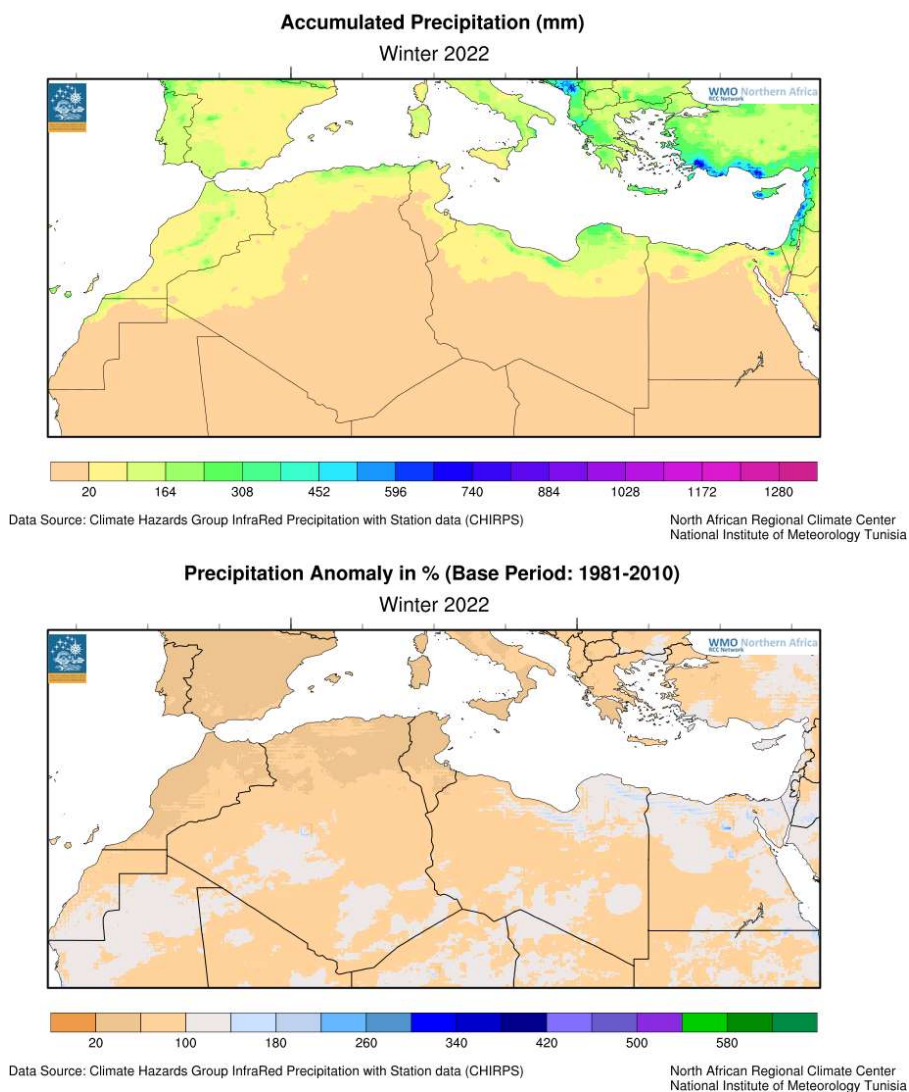
Figure 19: Winter (DJF 2021/22) precipitation totals and anomalies. Source: National Institute of Meteorology, Tunisia, https://www.meteo.tn/en/climate-monitoring-watch
