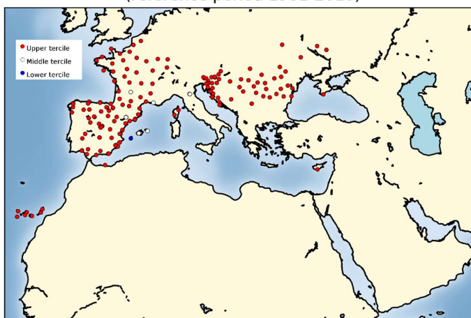
TEMPERATURE DJF 2021-2022 (ECA&D data) (reference period 1981-2010)
