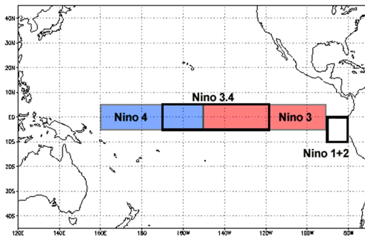
Figure 3: Definition of Niño regions, source: NOAA, https://www.ncei.noaa.gov/access/monitoring/enso/sstoi#oni
