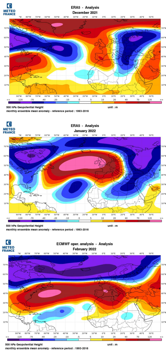
Figure 7: Monthly anomalies of 500-hPa geopotential for the months of winter 2021/22 (1993-2016 reference). Source: Météo France, data source: ECMWF / ERA5 reanalysis, http://seasonal.meteo.fr/content/suivi-clim-cartes-ref93-16 . Lower maps: same for individual months.
