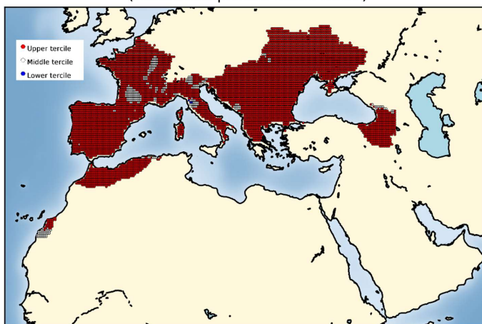
TEMPERATURE DJF 2021-2022 (EOBS data) (reference period 1981-2010)
