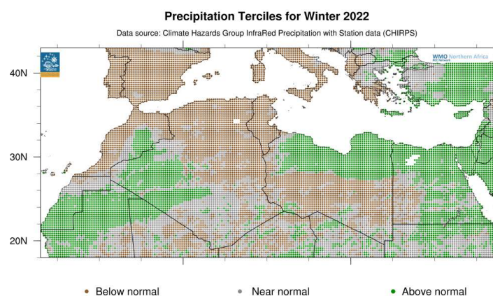
Figure 20: Precipitation terciles for 2021/2022 winter season in North Africa (Reference period 1981-2010). Source: National Institute of Meteorology, Tunisia
