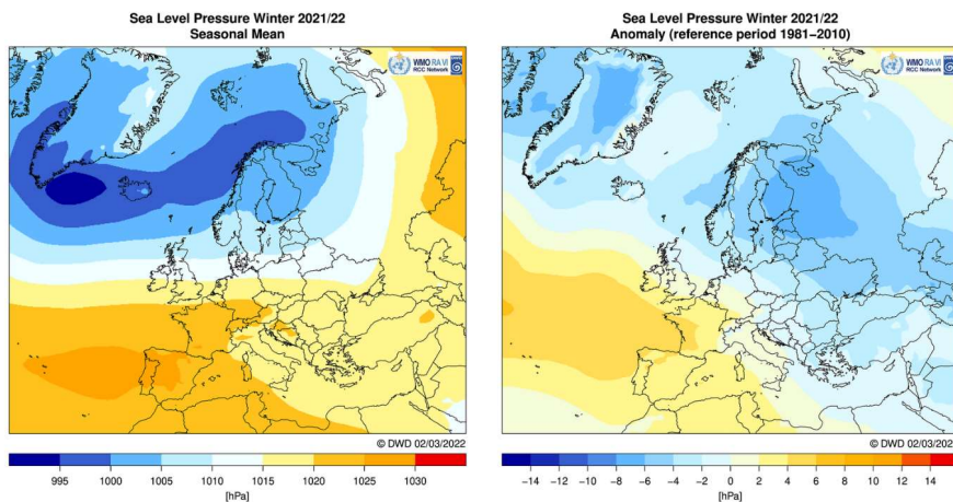
Figure 8: Seasonal mean sea level pressure and its anomalies for winter 2021/22 (1981-2010 reference). Source: Deutscher Wetterdienst (DWD), https://www.dwd.de/EN/ourservices/rcccm/int/rcccm_int_ppp.html , data source: DWD numerical ICON model analysis, http://www.dwd.de/EN/research/weatherforecasting/num_modelling/01_num_weather_prediction_modells/icon_description.html?nn=484268
