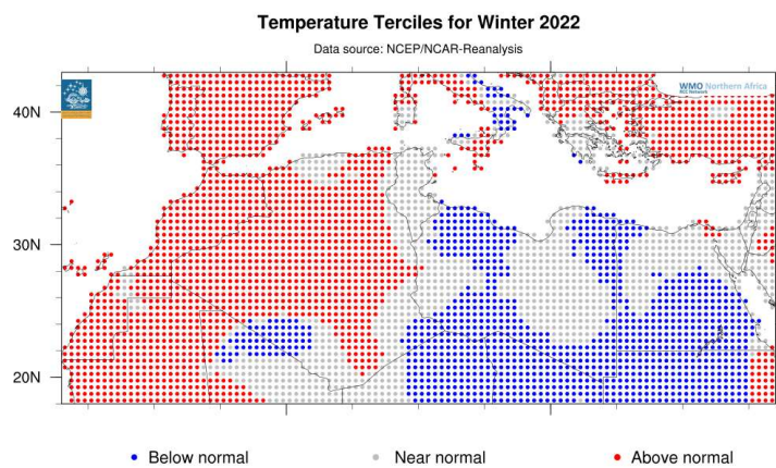
Figure 15: Temperature terciles for the 2021/2022 winter season in North Africa (Reference period 1981-2010). Source: National Institute of Meteorology, Tunisia
