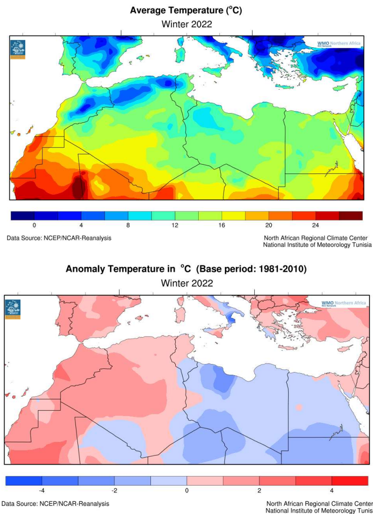
Figure 14: Winter (DJF 2021/22) mean temperatures and anomalies. Source: National Institute of Meteorology, Tunisia, https://www.meteo.tn/en/climate-monitoring-watch
