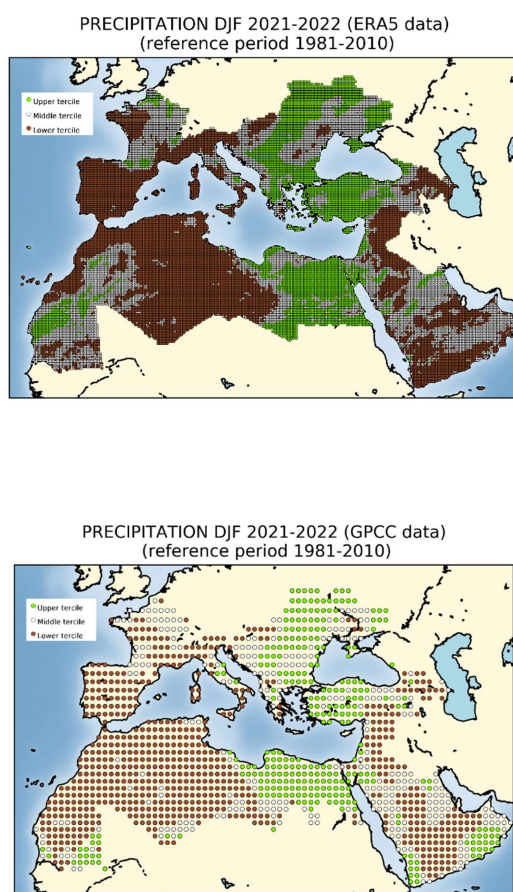
Figure 17: Terciles of winter 2021/22 precipitation based on ERA5 reanalysis (upper graph) and GPCC (lower graph) grid data, 1981-2010 reference. Source: AEMET, data reference: ERA5: https://www.ecmwf.int/en/forecasts/datasets/reanalysis-datasets/era5 , GPCC: http://gpcc.dwd.de
