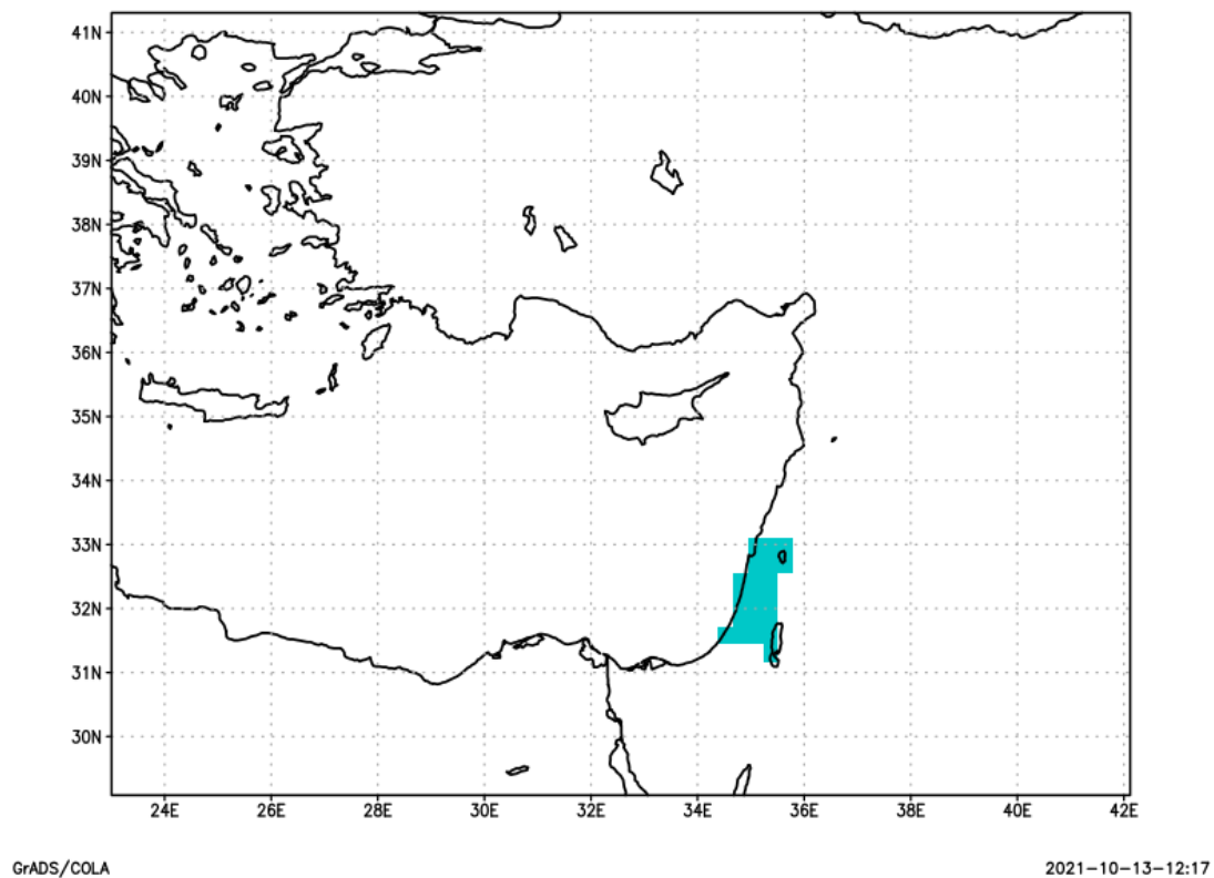
Figure 4: The area of 20 grid points which are used in order to make precipitation seasonal forecast for DJF season in Israel.
