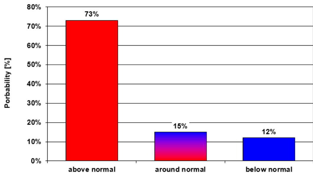
Figure 1: The probabilities for the 3 temperature terciles over Israel for winter 2021/22 (DJF 2021/22).
