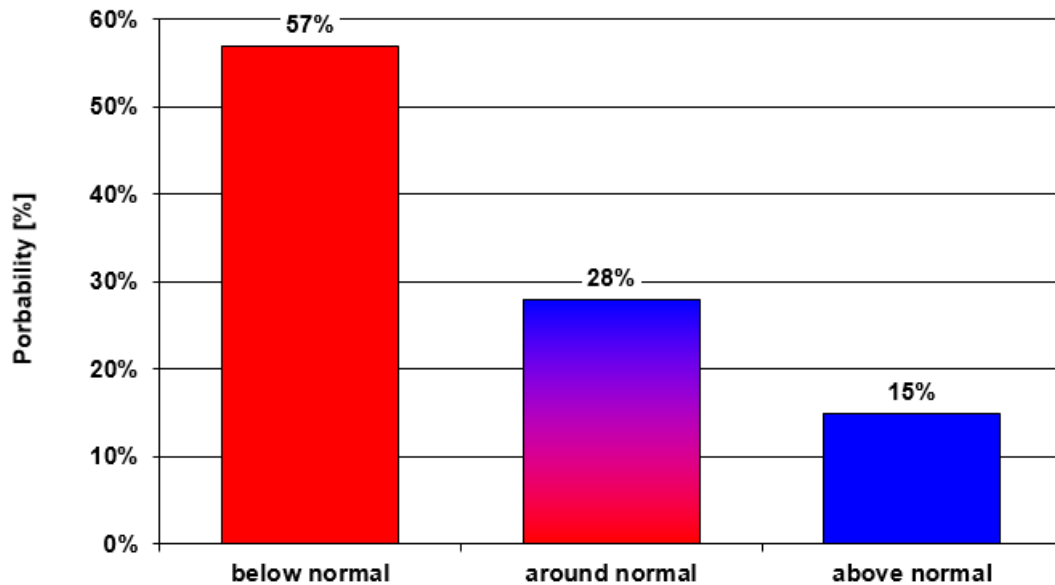
Figure 3: The probabilities for the 3 precipitation terciles over Israel for winter 2021/22.
