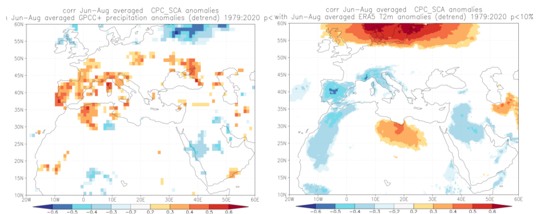
Figure 3. JJA Scand impact on precipitation (left) and temperature (right)
