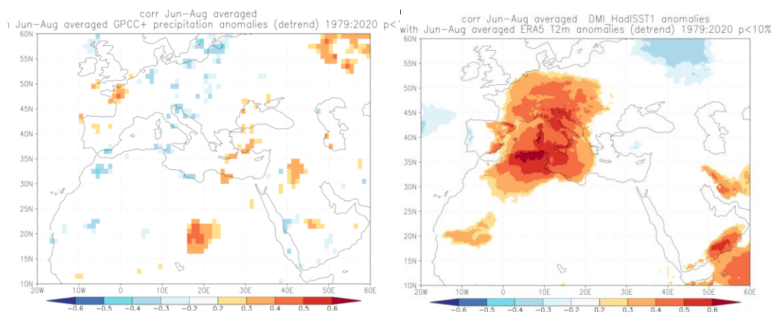
Figure 5. JJA DMI impact on precipitation (left) and temperature (right)
