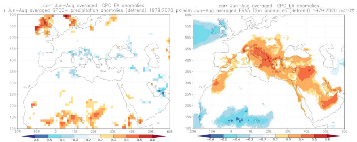
Figure 2. JJA EA impact on precipitation (left) and temperature (right)
