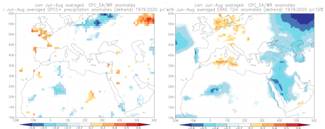
Figure 4. JJA EA/WR impact on precipitation (left) and temperature (right)
