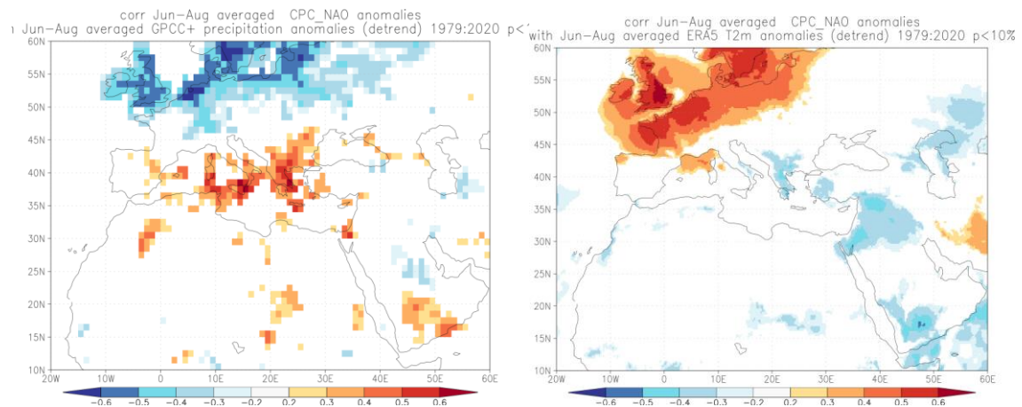
Figure 1. JJA NAO impact on precipitation (left) and temperature (right)
