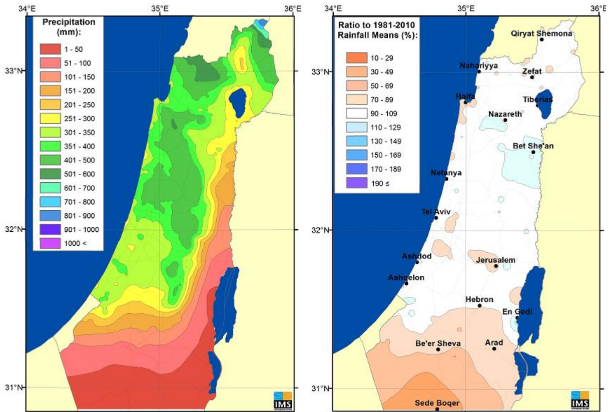
Fig 4. (a) DJF 2020/21 accumulated precipitation (mm). (b) Percent of normal (1981-2010).
