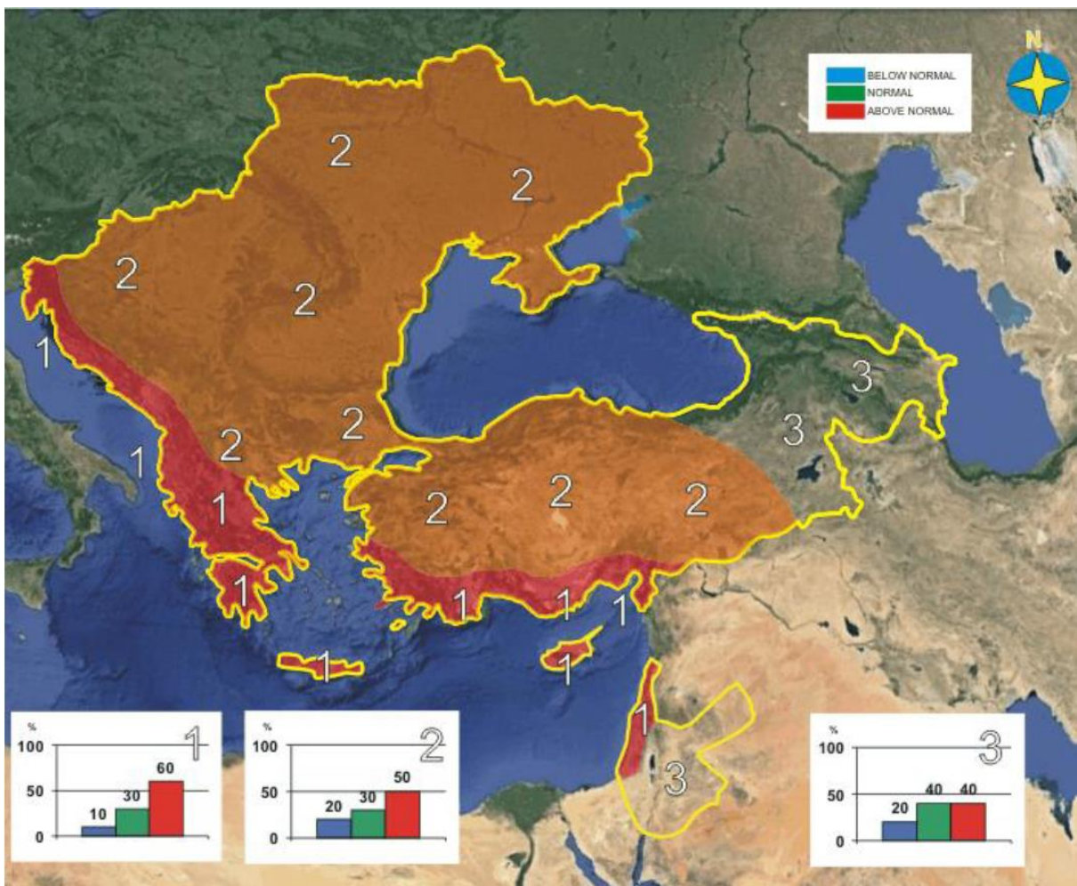
Fig 1. SEECOF-24 temperature outlook for 2020-2021.
