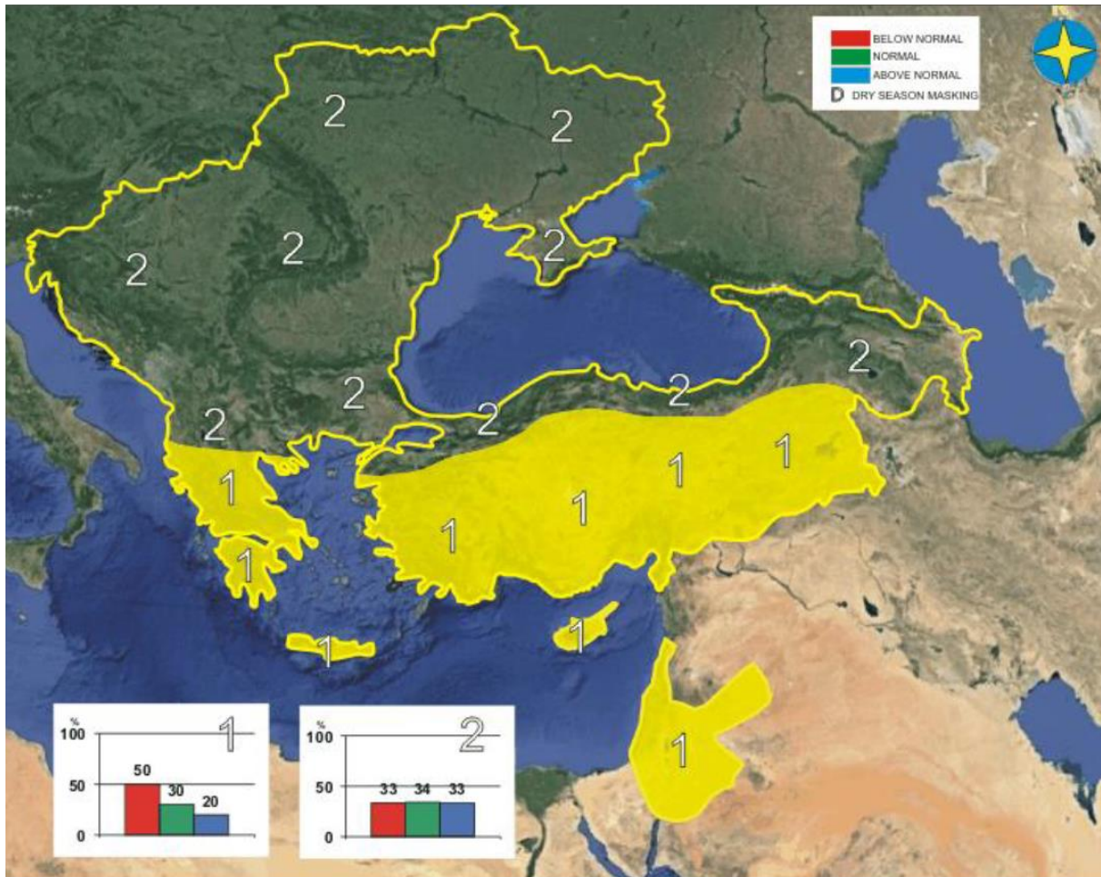
Fig 2. SEECOF-24 precipitation outlook for 2020-2021.
