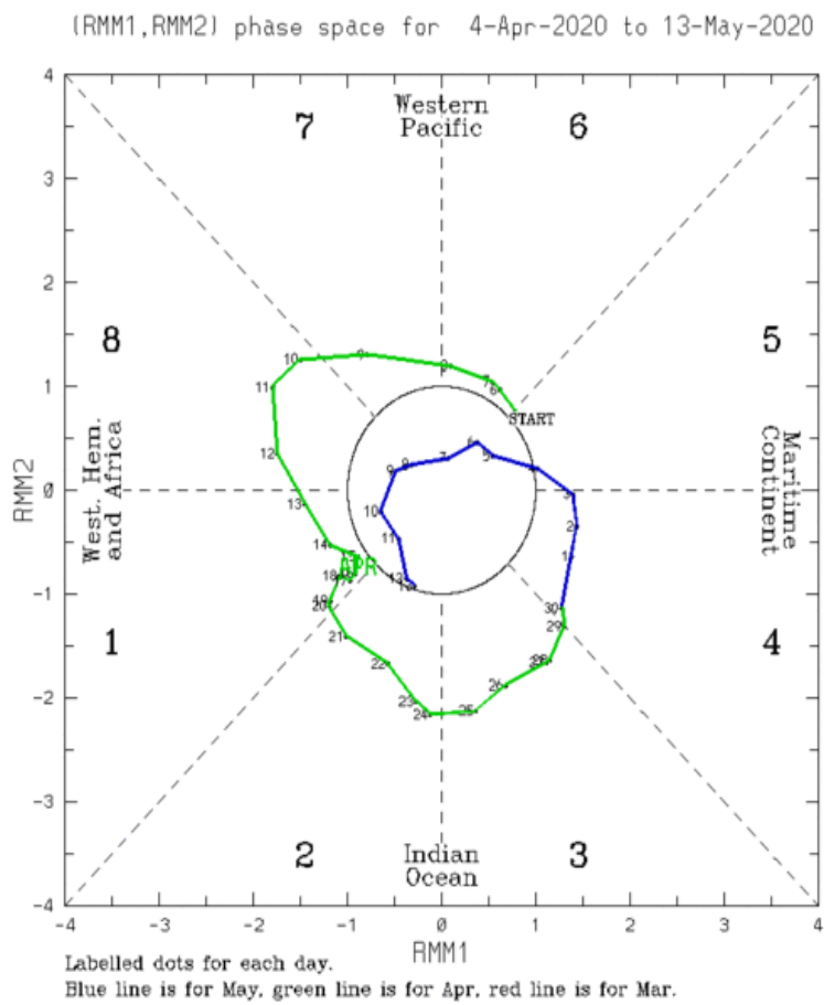
Figure 2.1.b: indices MJO
