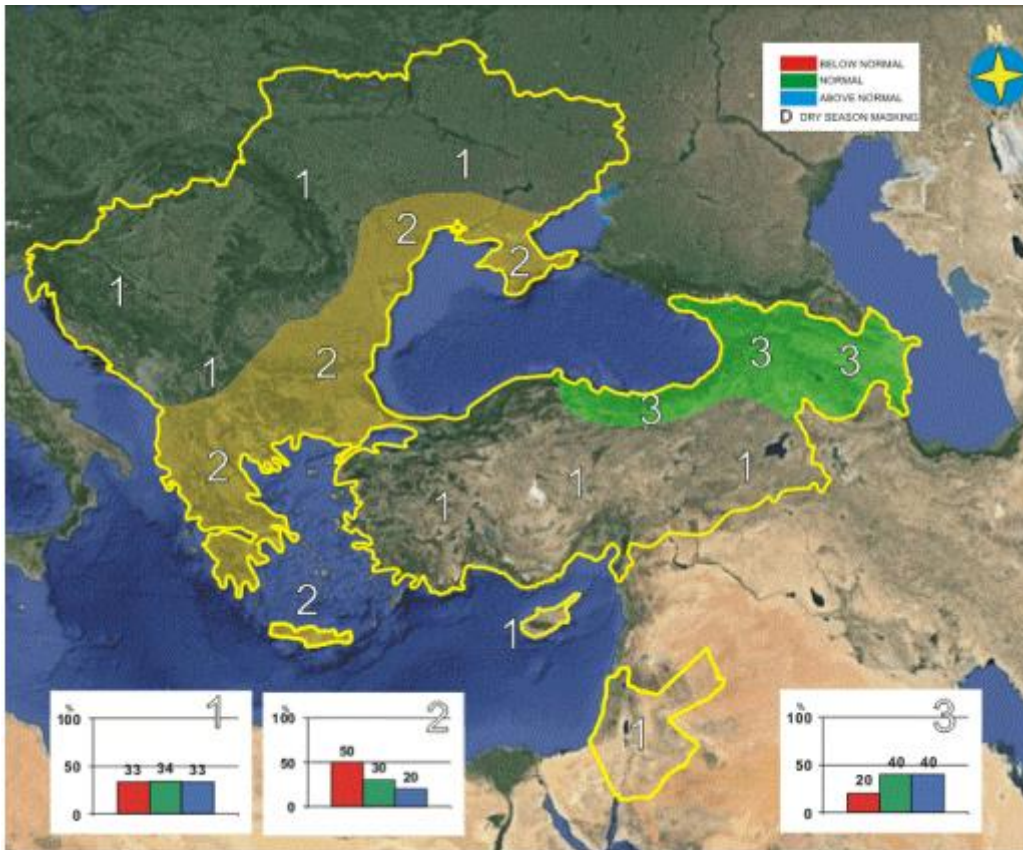
Fig 2. SEECOF-22 precipitation outlook for 2019-2020.
