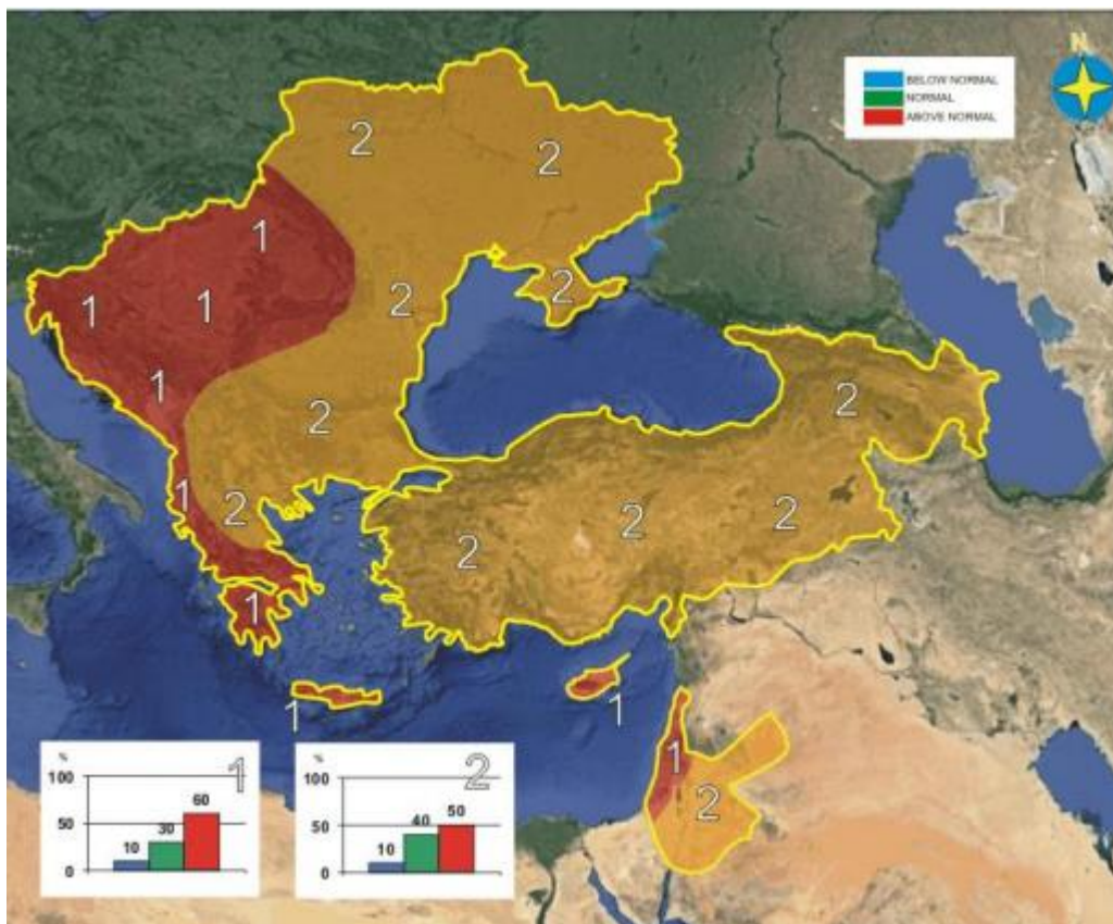
Fig 1. SEECOF-22 temperature outlook for 2019-2020.
