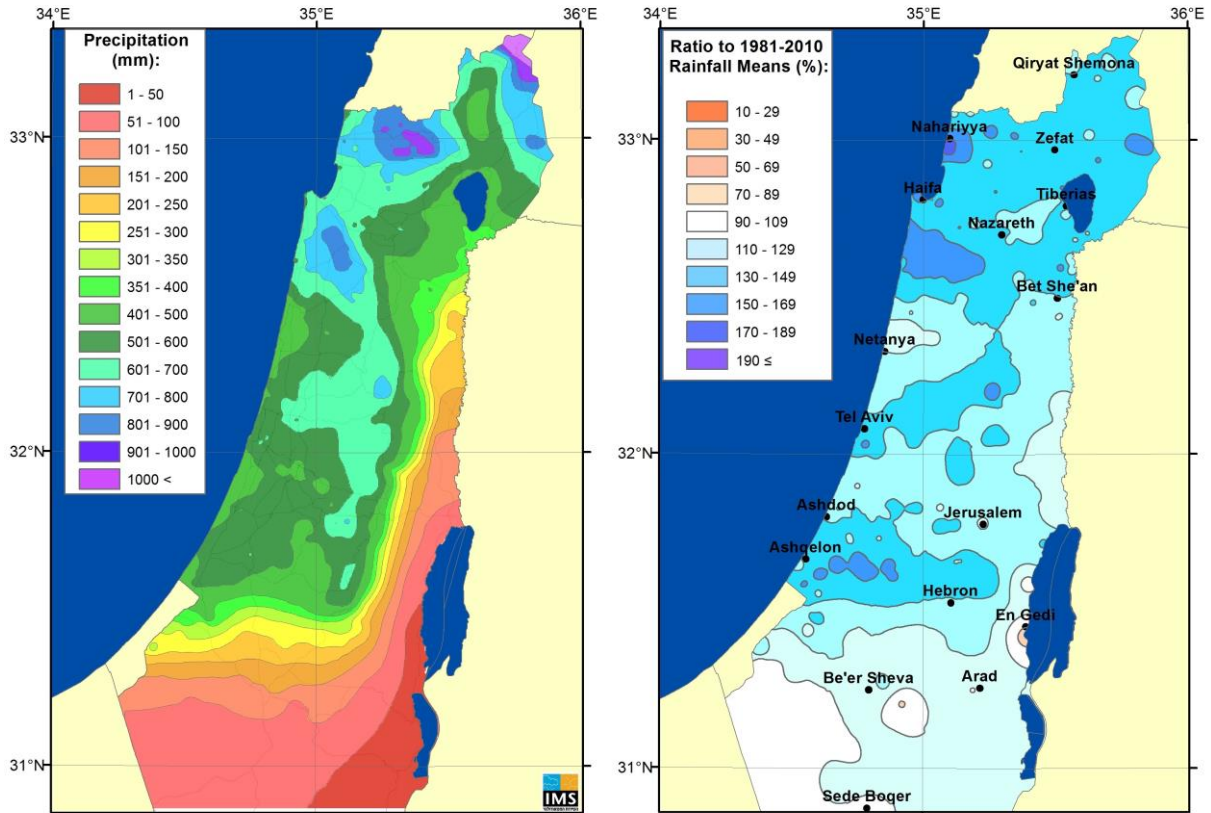
Fig 4. (a) DJF 2019/20 accumulated precipitation (mm). (b) Percent of normal (1981-2010).
