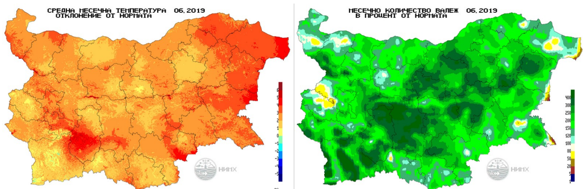
Figure 2: Departure of the monthly mean temperature from normal (1961-1990) (left) and monthly amount of precipitation in percent of normal (1961-1990) (right) for June 2019.
