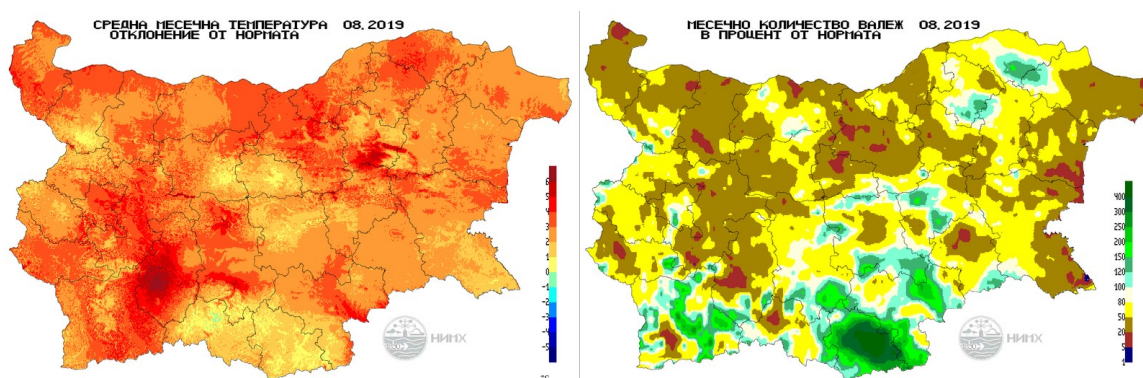
Figure 4: Departure of the monthly mean temperature from normal (1961-1990) (left) and monthly amount of precipitation in percent of normal (1961-1990) (right) for August 2019.
