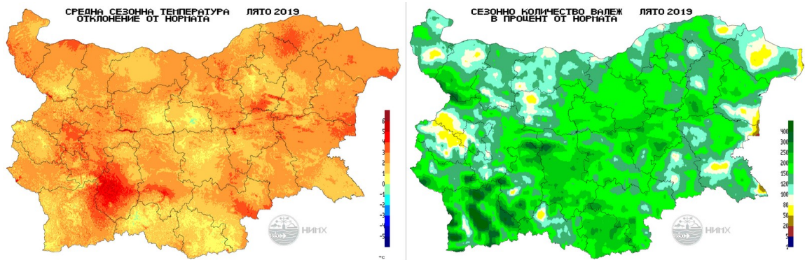
Figure 1: Departure of the seasonal mean temperature from normal (1961-1990) (left) and seasonal amount of precipitation in percent of normal (1961-1990) (right) for summer (June-July-August) 2019.
