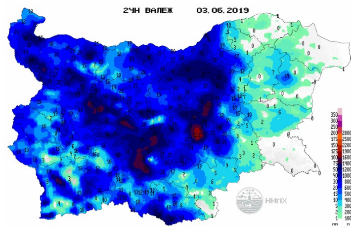
Figure 6: 24-hour precipitation amount for 3 June 2019.
