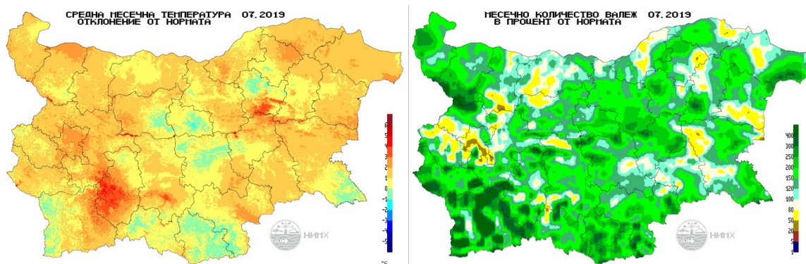
Figure 3: Departure of the monthly mean temperature from normal (1961-1990) (left) and monthly amount of precipitation in percent of normal (1961-1990) (right) for July 2019.
