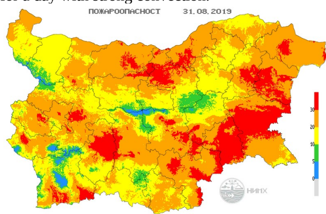
Figure 5: Fire weather index on 31 August 2019.
