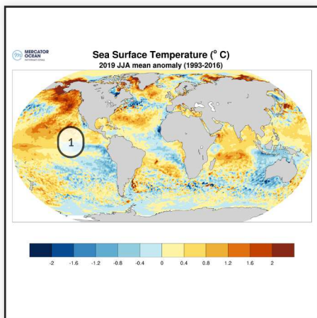
1- Negative anomaly observed while it was expected positive
