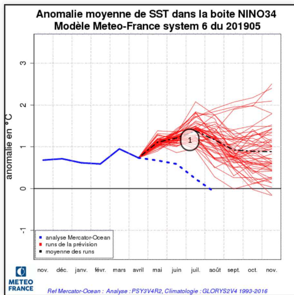
1- plume entirely above observation
