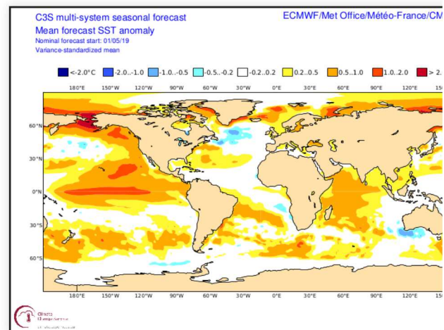
1- Negative anomaly observed while it was expected positive
