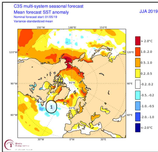
1- the cold anomaly was predicted too far north and not extended enough eastward.
