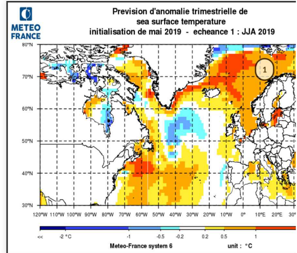
1- Norwegian sea predicted too hot
