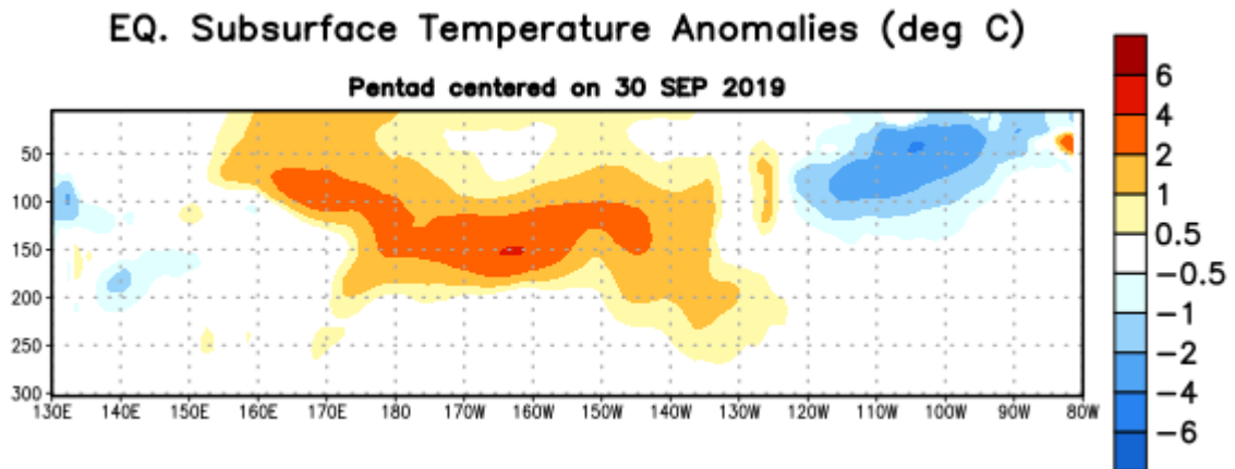
Figure 4. Depth-longitude section of equatorial Pacific upper-ocean (0-300m) temperature anomalies ( ^{\circ}\text{C} ) centered on the pentad of 30 September 2019. Anomalies are departures from the 1981-2010 base period pentad means.
