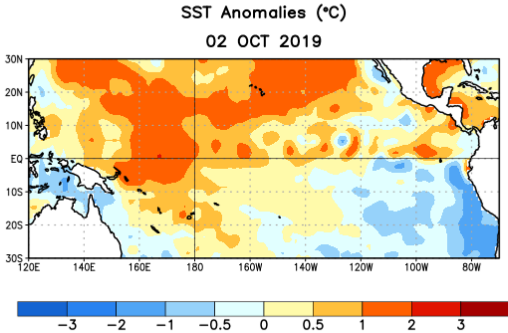
Figure 1. Average sea surface temperature (SST) anomalies (°C) for the week centered on 2 October 2019. Anomalies are computed with respect to the 1981-2010 base period weekly means.
