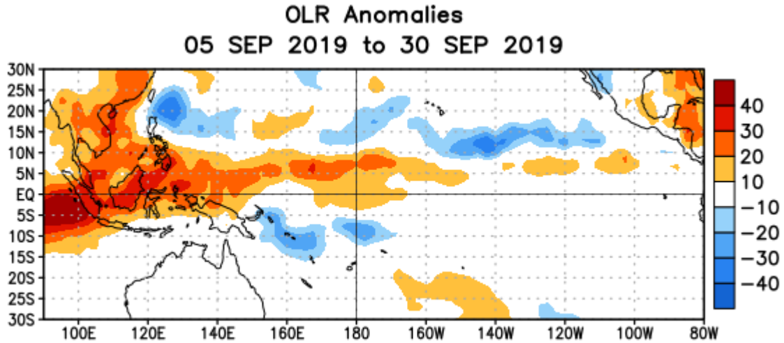
Figure 5. Average outgoing longwave radiation (OLR) anomalies ( \text{W/m}^2 ) for the period 5 – 30 September 2019. OLR anomalies are computed as departures from the 1981-2010 base period pentad means.
