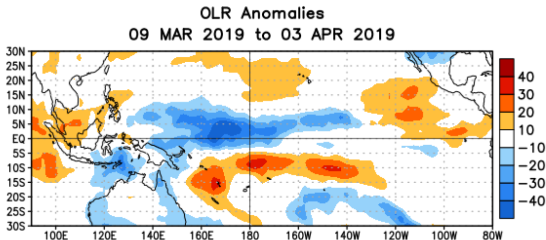
Figure 5. Average outgoing longwave radiation (OLR) anomalies ( \text{W/m}^2 ) for the period 9 March – 3 April 2019. OLR anomalies are computed as departures from the 1981-2010 base period pentad means.
