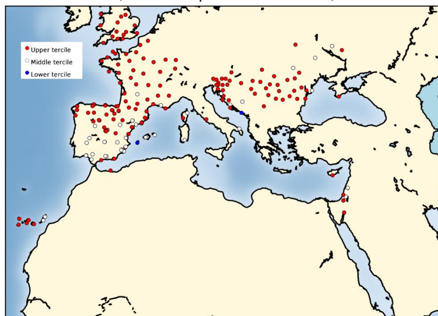
TEMPERATURE DJF 2019 (ECA&D data) (reference period 1981-2010)
