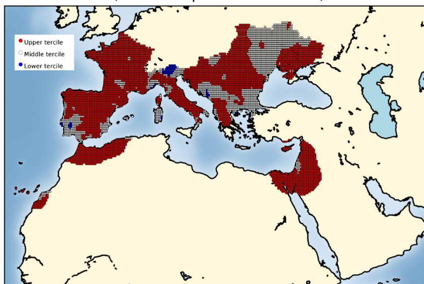
TEMPERATURE DJF 2019 (EOBS data) (reference period 1981-2010)
