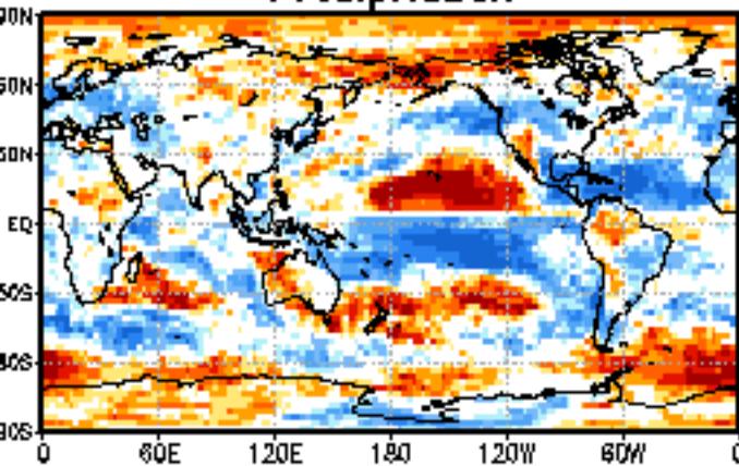
Precipitation
