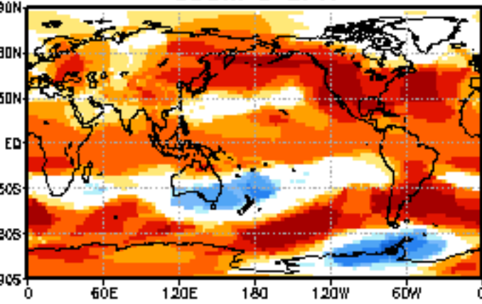
500hPa GPH
