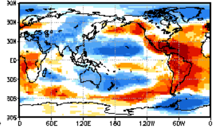
Mean Sea Level Pressure
