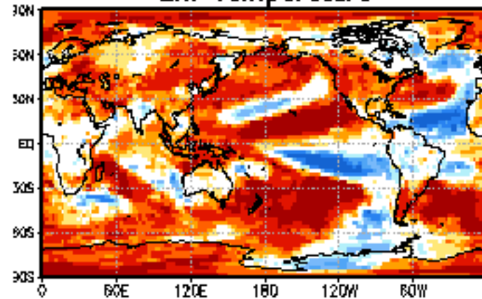
2m Temperature
