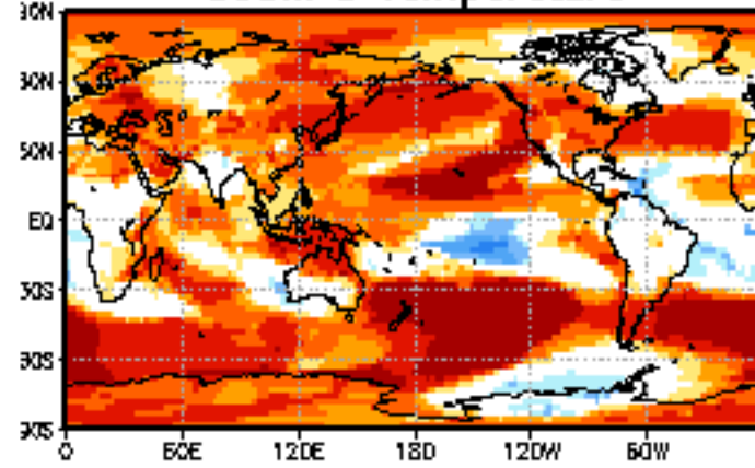
850hPa Temperature
