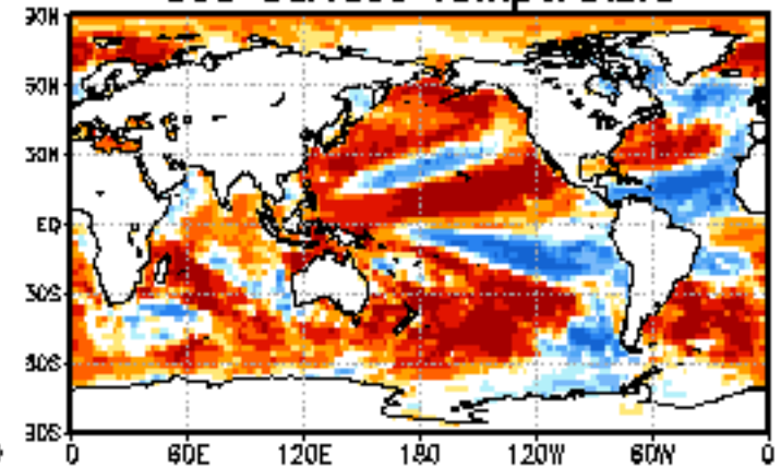
Sea Surface Temperature
