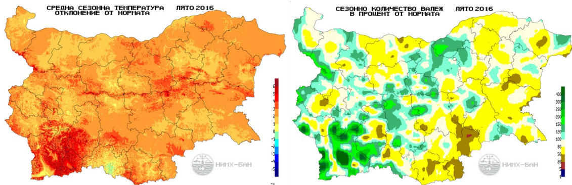
Figure 1: Departure of the seasonal mean temperature from normal (1961-1990) (left) and seasonal amount of precipitation in percent of normal (1961-1990) (right) for summer (June-July-August) 2016.
