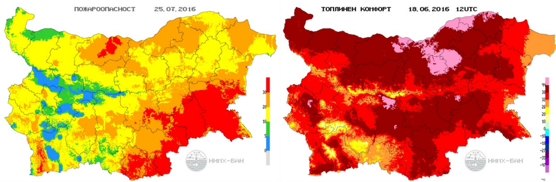
Figure 5: (a) Fire weather index on 25 July 2016; (b) Perceived temperature in categories of human thermal comfort on 18 June 2016 12UTC (15h local summer time).
