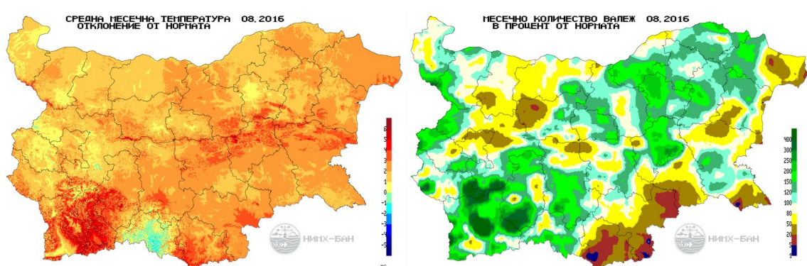
Figure 4: Departure of the monthly mean temperature from normal (1961-1990) (left) and monthly amount of precipitation in percent of normal (1961-1990) (right) for August 2016.
