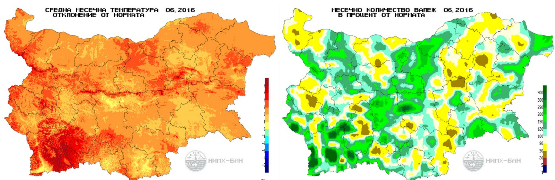
Figure 2: Departure of the monthly mean temperature from normal (1961-1990) (left) and monthly amount of precipitation in percent of normal (1961-1990) (right) for June 2016.
