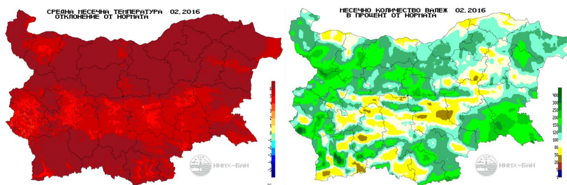
Figure 3: Departure of the monthly mean temperature from normal (1961-1990) (left) and monthly amount of precipitation in percent of normal (1961-1990) (right) for February 2016.
