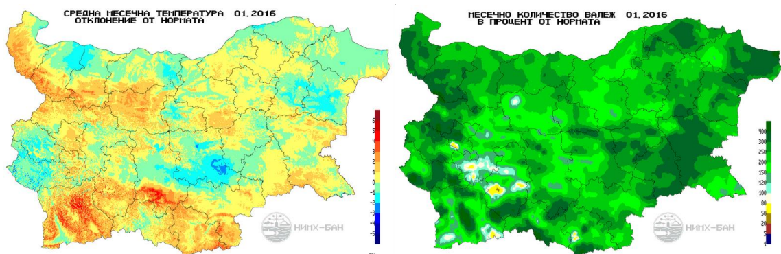
Figure 2: Departure of the monthly mean temperature from normal (1961-1990) (left) and monthly amount of precipitation in percent of normal (1961-1990) (right) for January 2016.
