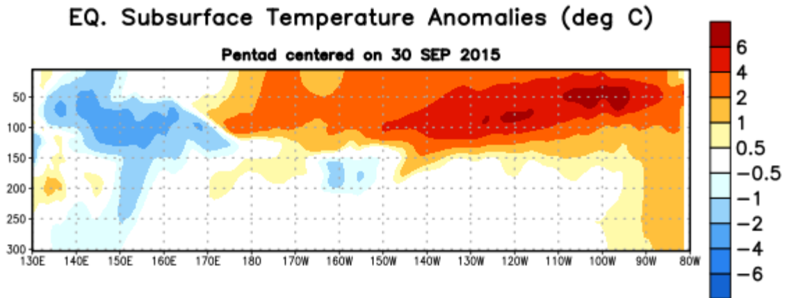
Figure 4. Depth-longitude section of equatorial Pacific upper-ocean (0-300m) temperature anomalies ( ^{\circ}\text{C} ) centered on the pentad of 30 September 2015. The anomalies are averaged between 5^{\circ}\text{N} - 5^{\circ}\text{S} . Anomalies are departures from the 1981-2010 base period pentad means.
