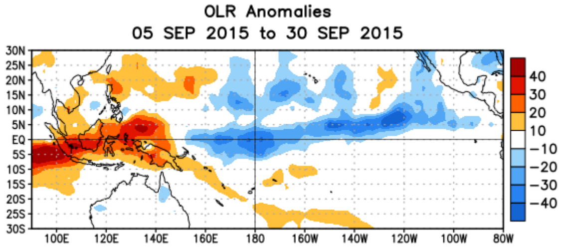
Figure 5. Average outgoing longwave radiation (OLR) anomalies ( W/m^2 ) for the period 5 – 30 September 2015. OLR anomalies are computed as departures from the 1979-1995 base period pentad means.
