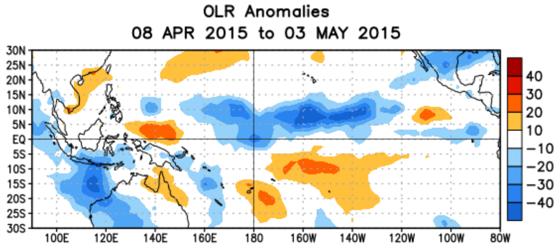
Figure 5. Average outgoing longwave radiation (OLR) anomalies ( \text{W/m}^2 ) for the period 8 April – 3 May 2015. OLR anomalies are computed as departures from the 1979-1995 base period pentad means.
