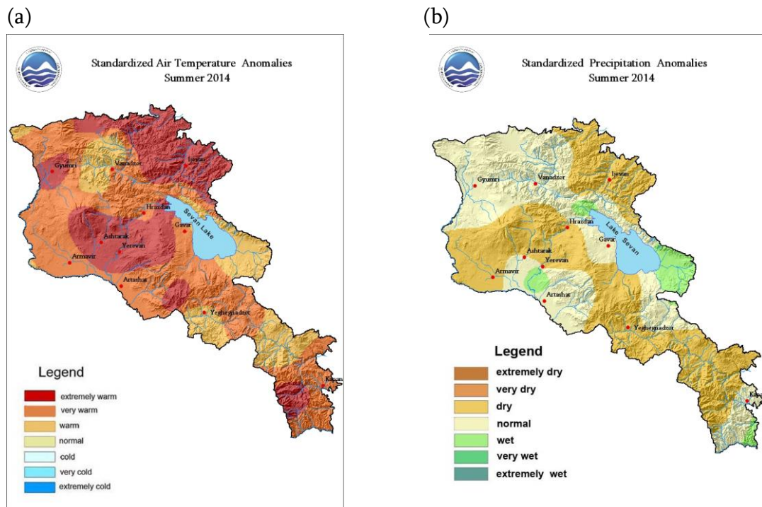
Figure 1. Anomalies of seasonal temperature (a) and precipitation (b) in summer 2014 over Armenia
