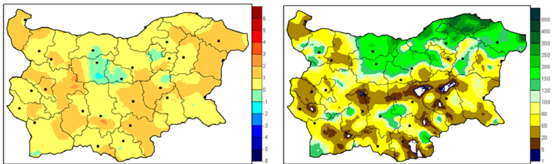
Figure 2: Departure of the monthly mean temperature from the norm (1961-1990) (left) and monthly amount of precipitation in percent of normal (1961-1990) (right) for June 2013.
