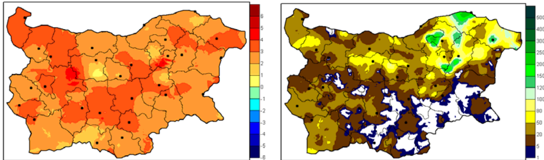
Figure 4: Departure of the monthly mean temperature from the norm (1961-1990) (left) and monthly amount of precipitation in percent of normal (1961-1990) (right) for August 2013.
