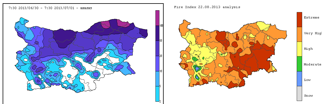
Figure 5: 24-hou precipitation amount, 01 July 2013 (left). Fire weather index, 22 August 2013 (right).
