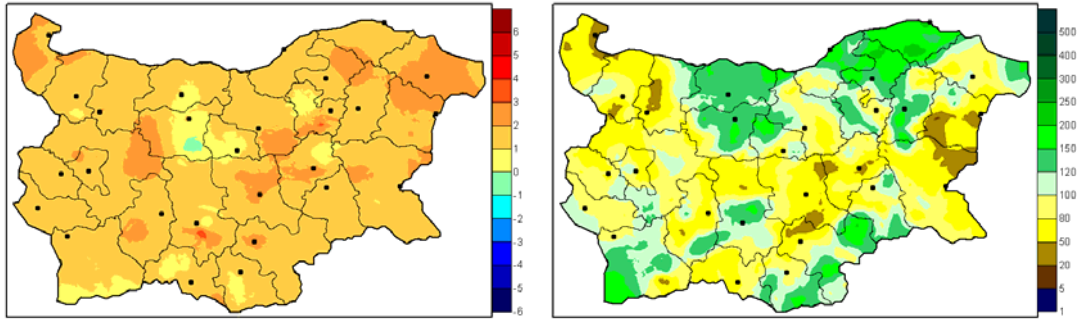
Figure 1: Departure of the monthly mean temperature from the norm (1961-1990) (left) and monthly amount of precipitation in percent of normal (1961-1990) (right) for summer (June-July-August) 2013.
