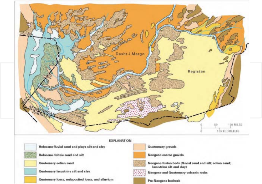
Figure 3. Geological map of the Sistan Basin and southern Afghanistan [61-63].
