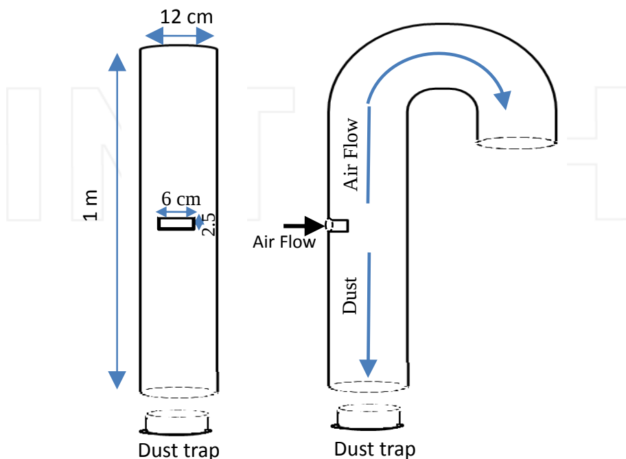
Figure 6. Schematic diagram of the dust sampler system.
