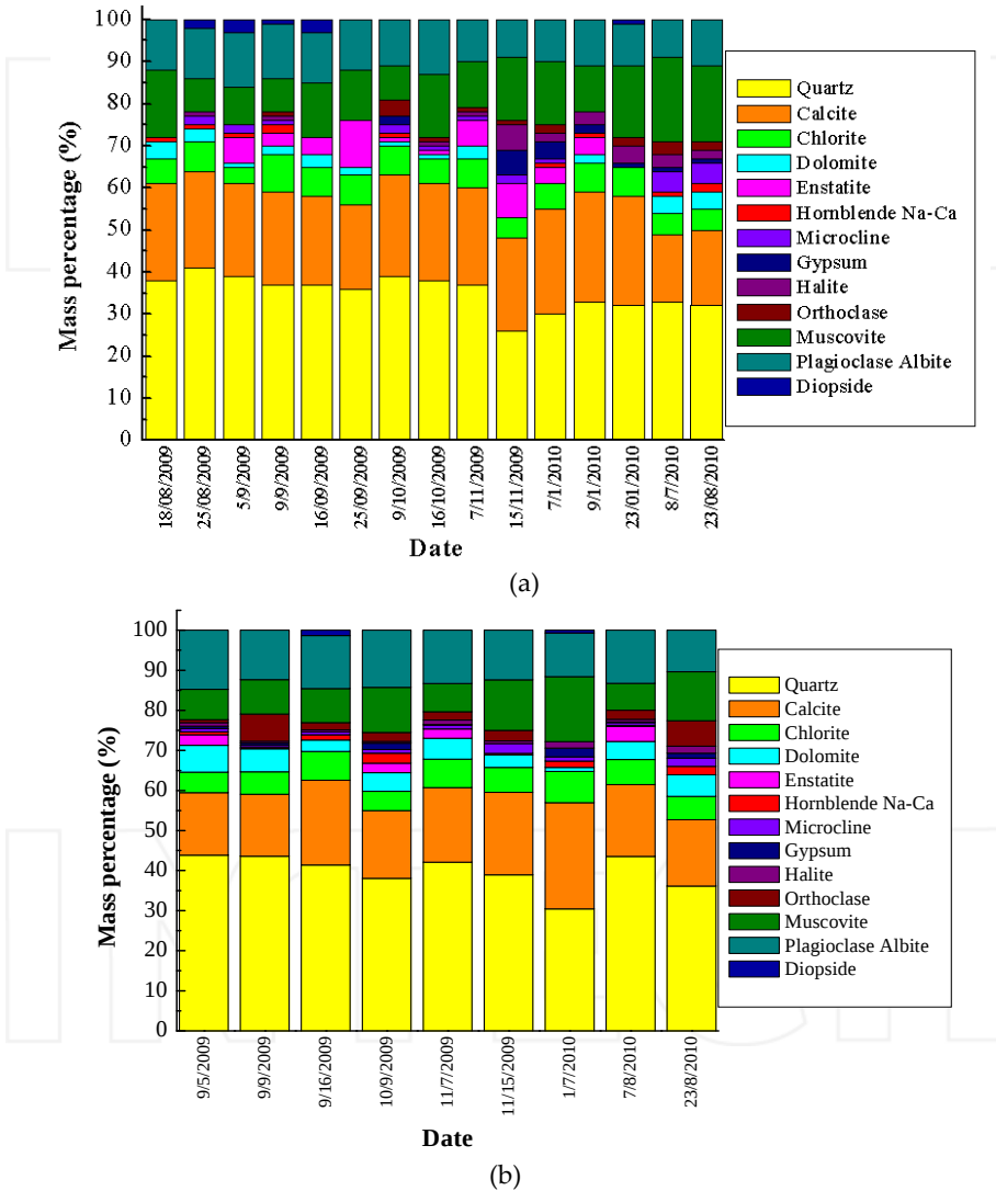
Figure 17. a. Mineralogical composition as obtained from XRD analysis for airborne dust samples collected on different days in station A. b. Same as in Figure 17a, but for the station B.
