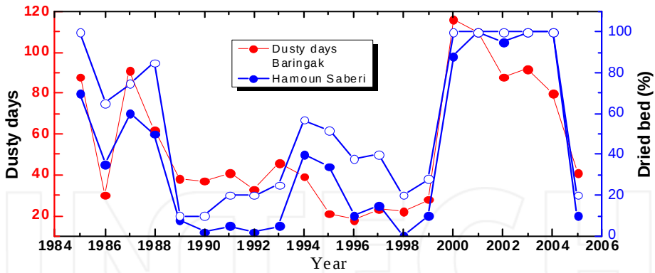
Figure 10. Yearly variability of the dusty days (visibility \leq 2\text{km} ) over Sistan region with association to percentage of Hamoun dried beds (1985-2005). The lower coverage of the Hamoun Basin by water (high percentage of dried beds) corresponds to higher number of dusty days over Sistan region.
