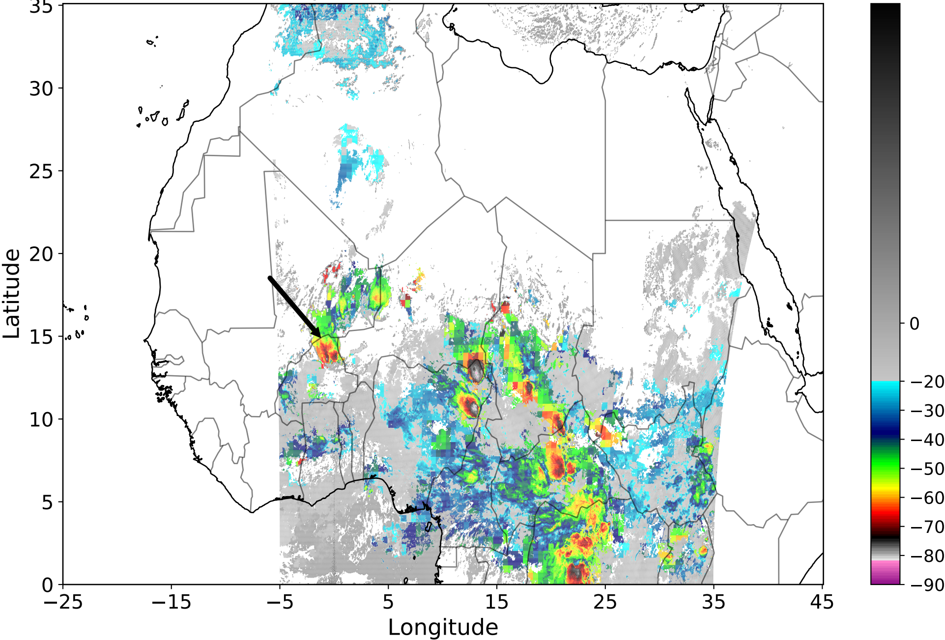
MSG-SEVIRI Cloud Top Temperature ( ° C) 2014-07-24 01:00 UTC
