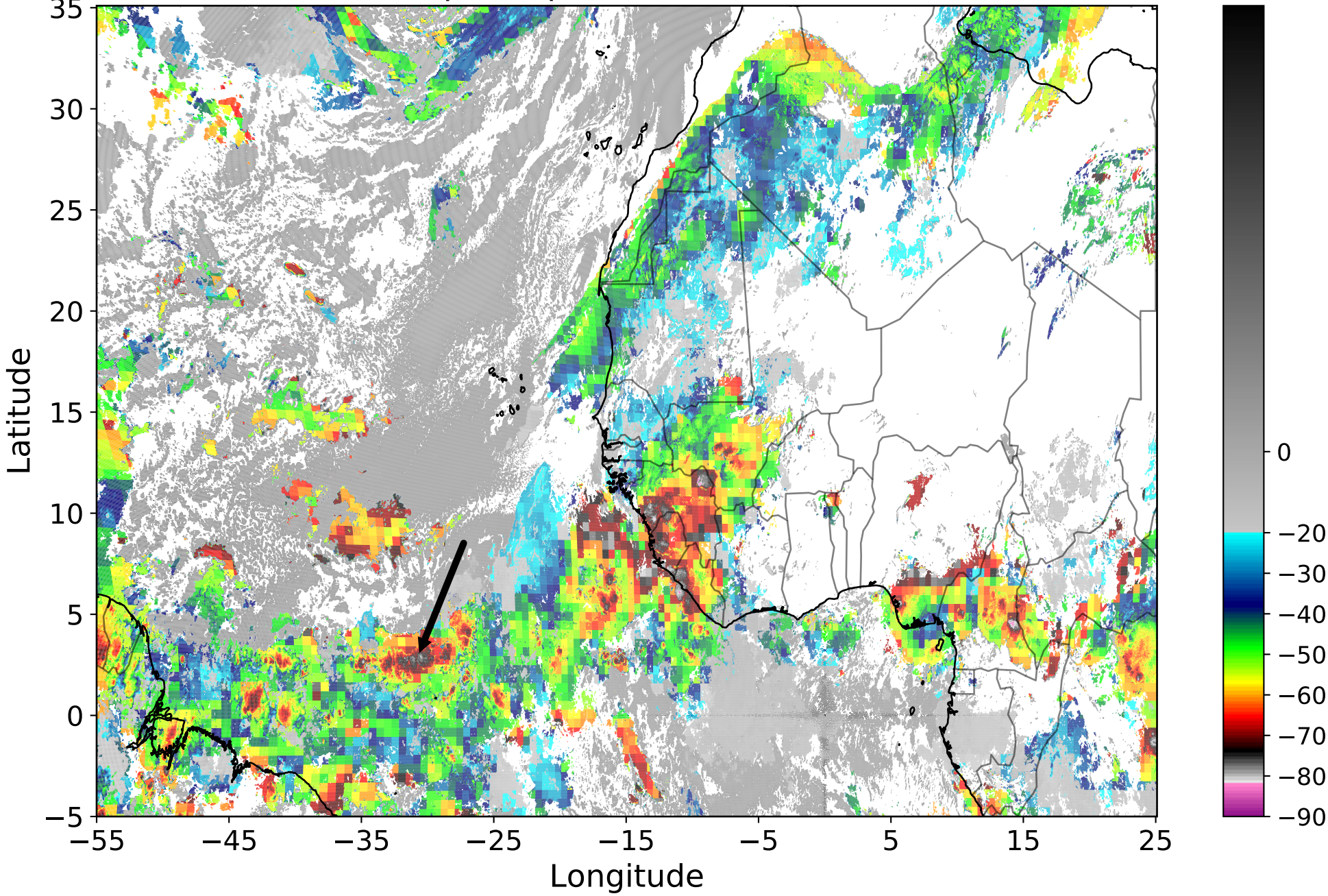
MSG-SEVIRI Cloud Top Temperature ( ° C) 2009-06-01 02:00 UTC
